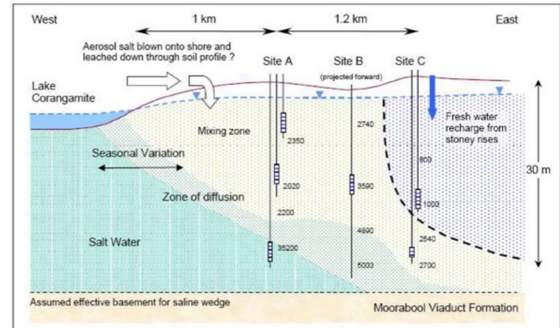
Figure 2 - Diagrammatical representation of a salt water wedge near Lake Corangamite showing groundwater salinities
