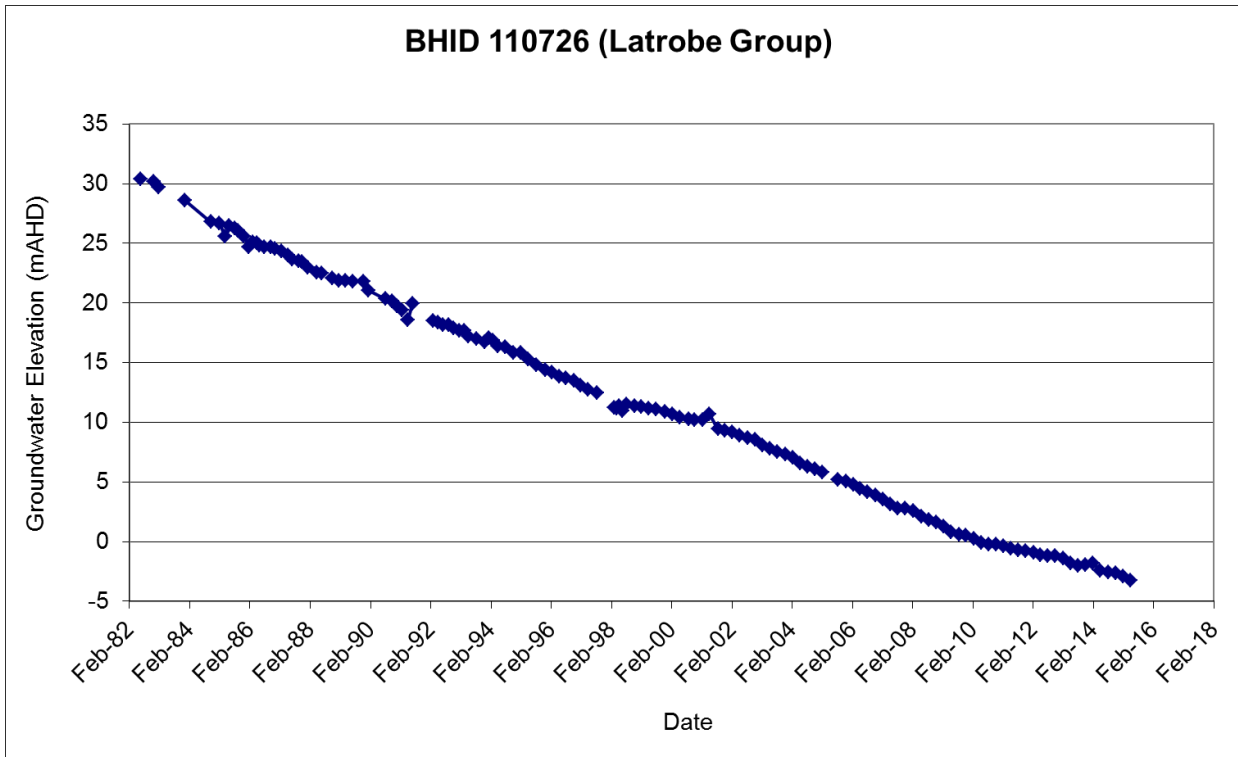
Figure 2: Example hydrograph
