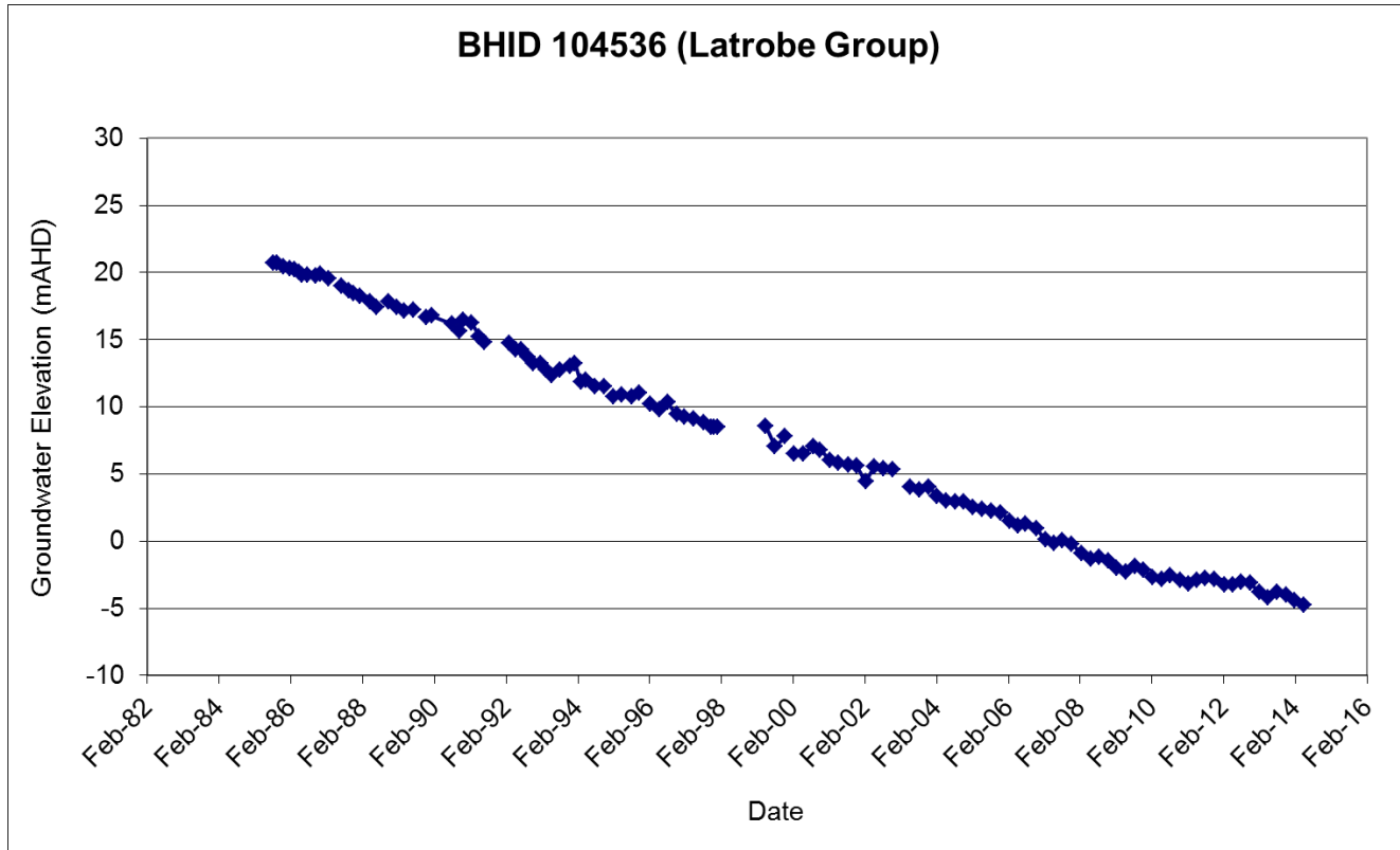
Figure 2: Example hydrograph
